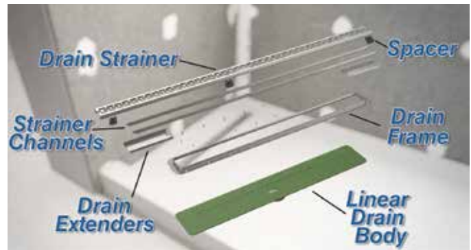
Figure 15: Drain assembly – exploded view
