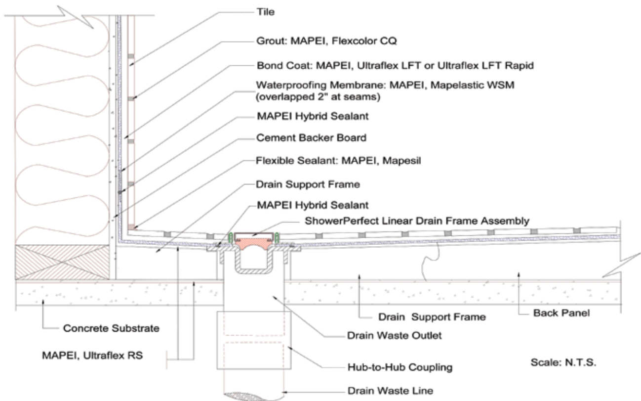
Figure 4: Drain orientation – set 3" to 6" (7,5 to 15 cm) from wall
