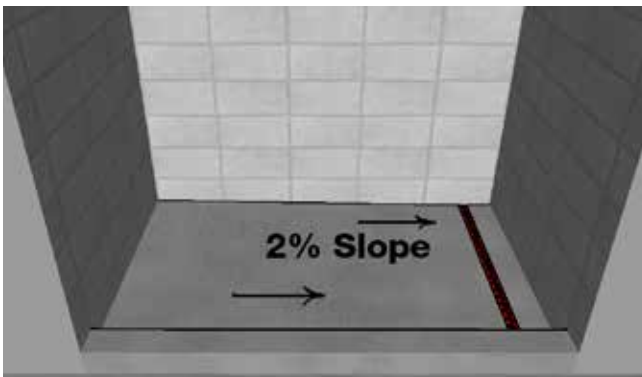
Figure 2: ShowerPerfect pre-sloped pan, 2% slope to drain
