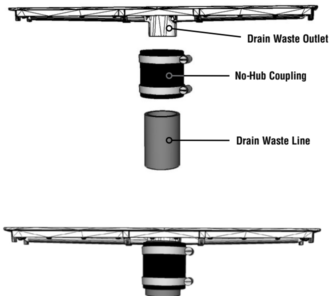
Figure 9: Attach the drain, no-hub coupling and 2" (5 cm) waste line (see Figure 4) – exploded view and assembled view
