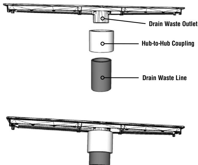
Figure 8: Clean, prime and glue the drain to the 2" (5 cm) waste line (see Figure 4) – exploded view and assembled view
