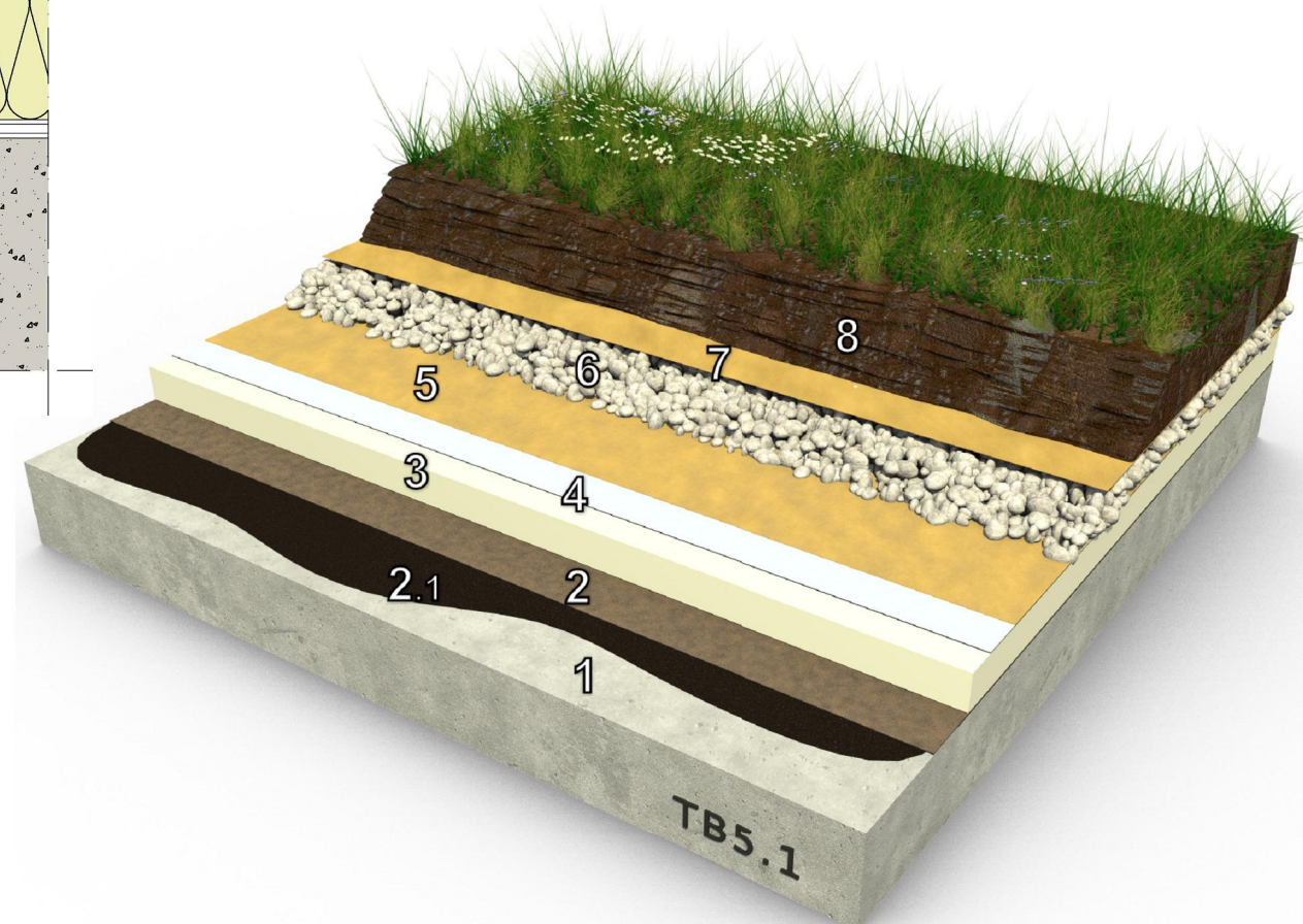
System TB5.1 Green roof with TPO/FPO synthetic waterproofing membrane (insulated)
